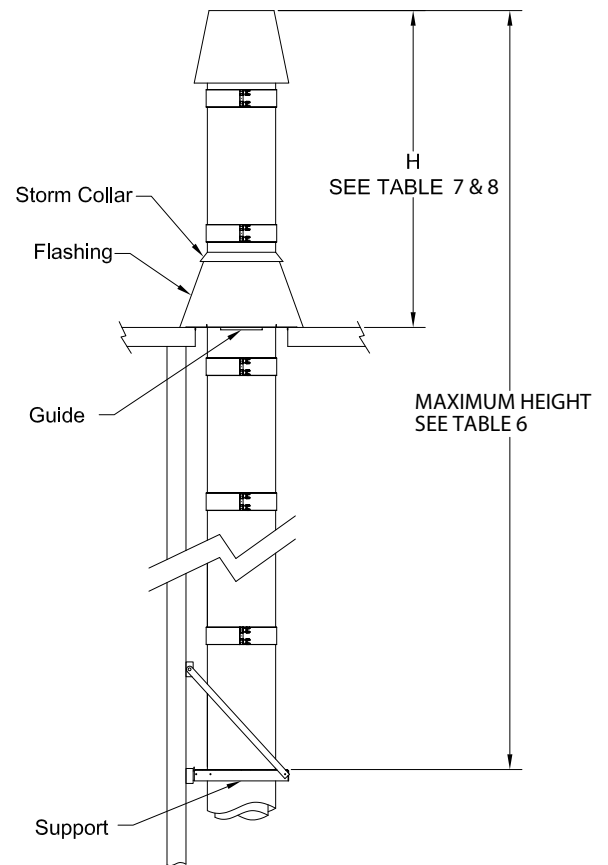
Figure 28- Maximum freestanding Height for LDCS & LDCD
