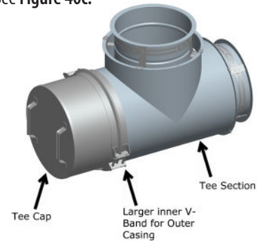
Figure 40c: Step 3-4 for installation of the LDCD TC
