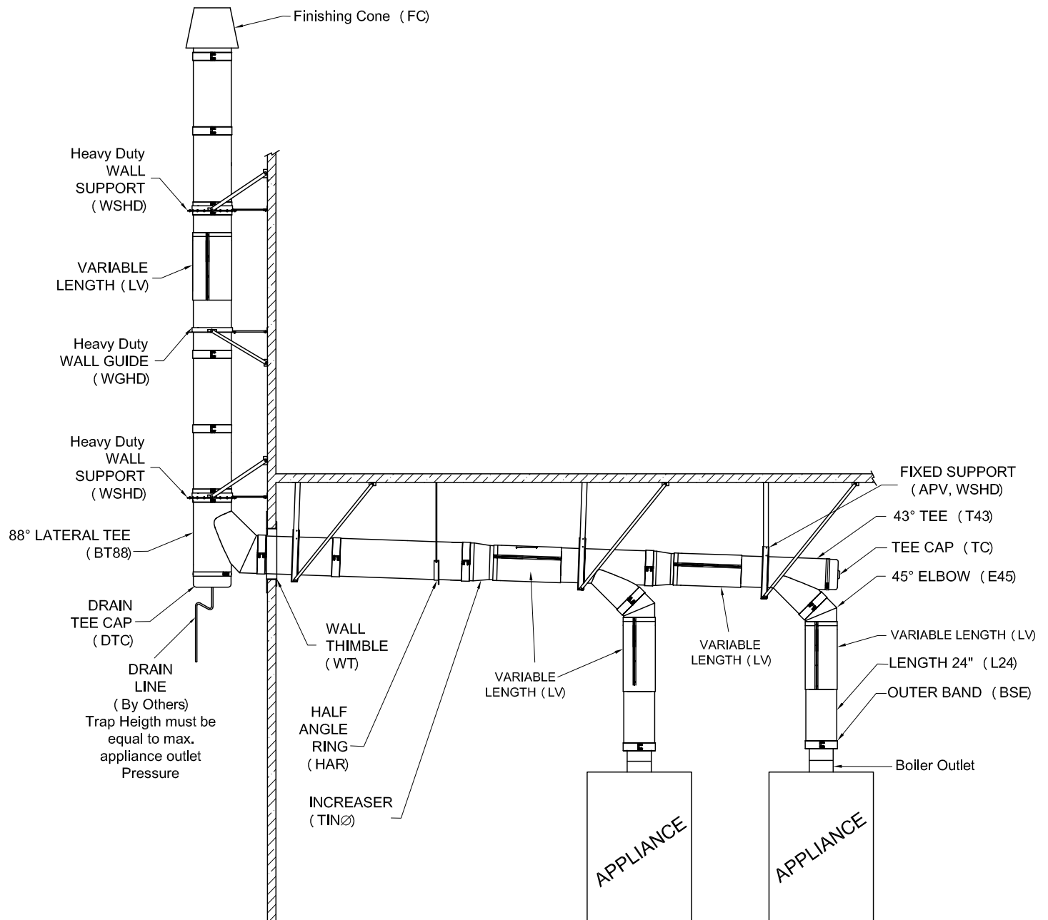
Figure 26- Typical installation for LDCD
