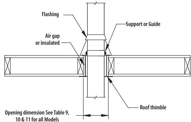
Figure 3 - Roof penetration
