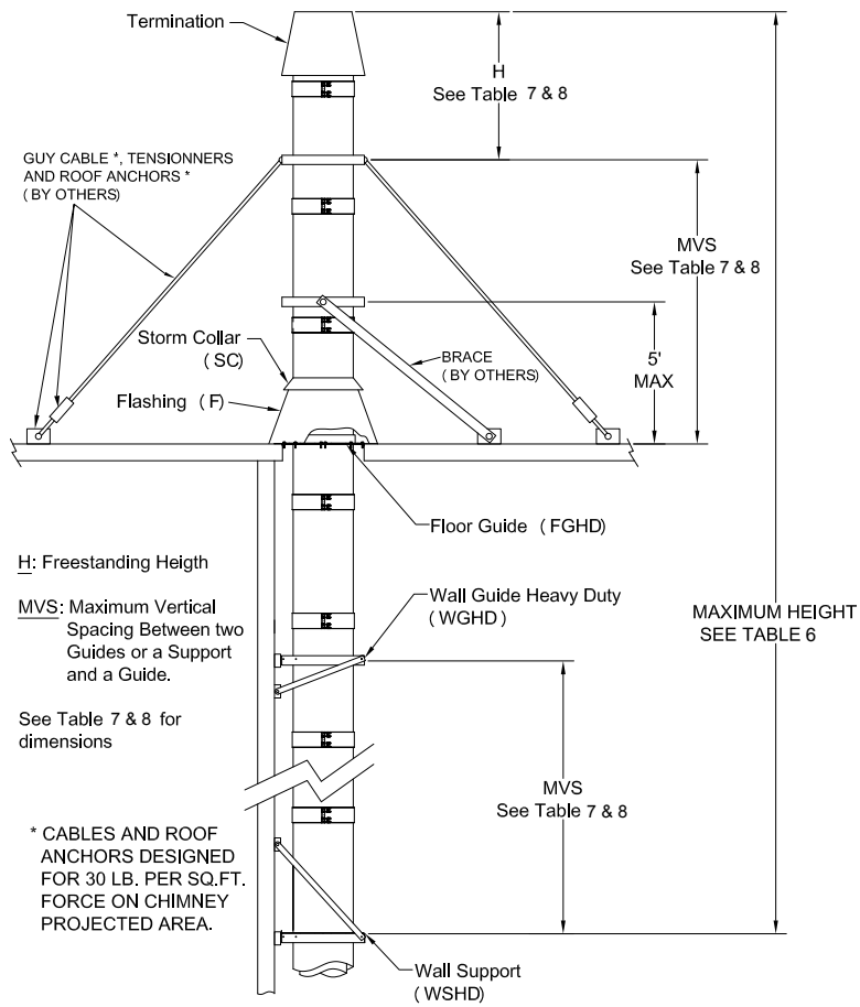
Figure 27 - Height with rigid bracing or guying option for LDCS & LDCD
