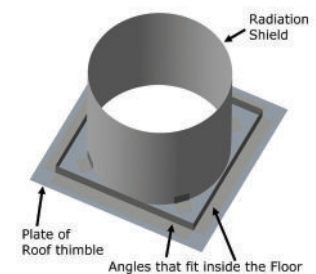
Figure 58a - Roof Thimble (RT)
